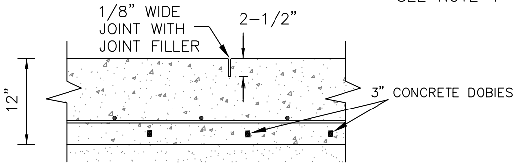
WEAKENED PLANE JOINT DETAIL
