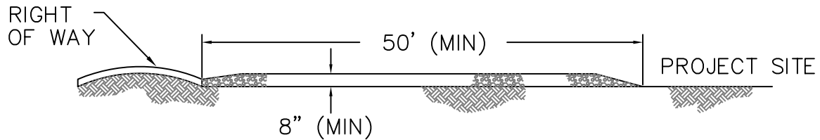
TYPICAL SECTION
